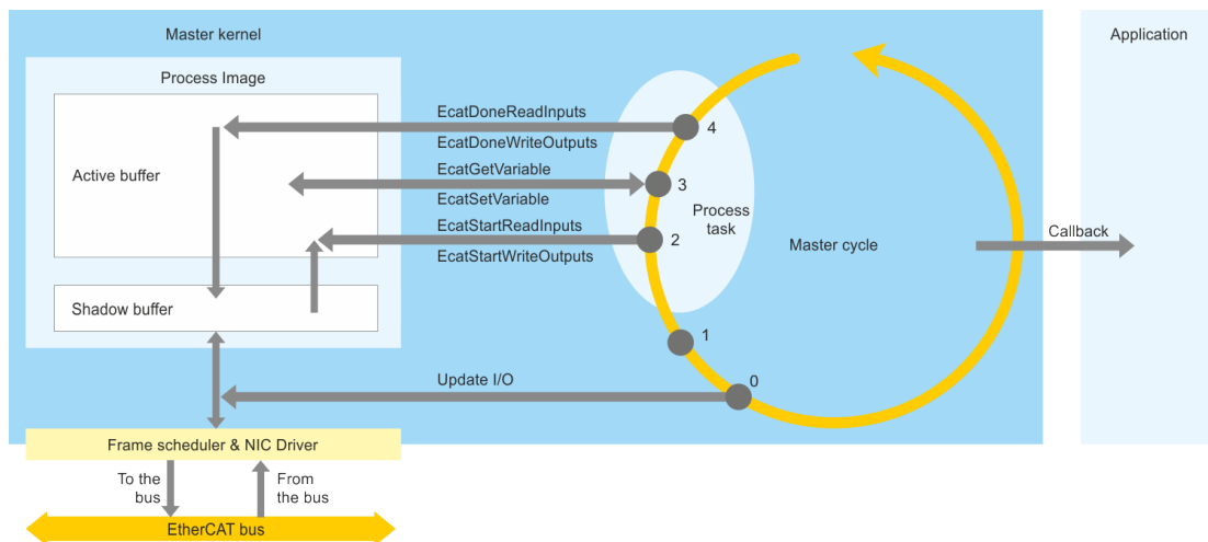
Figure 9. Synchronous mode
