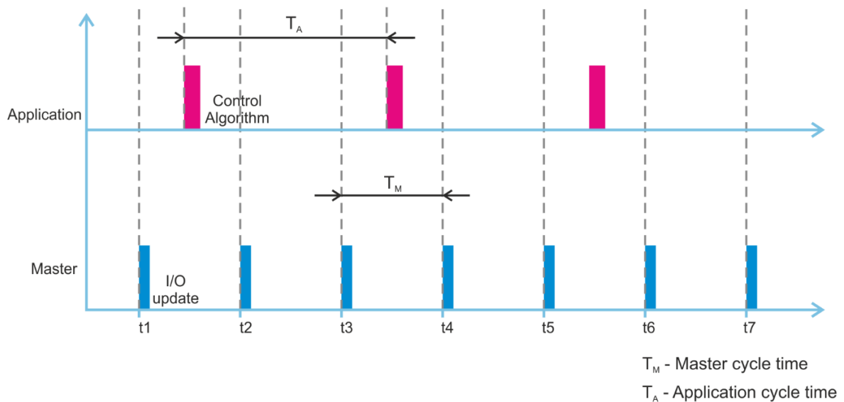
Figure 8. Timing chart of Asynchronous mode
