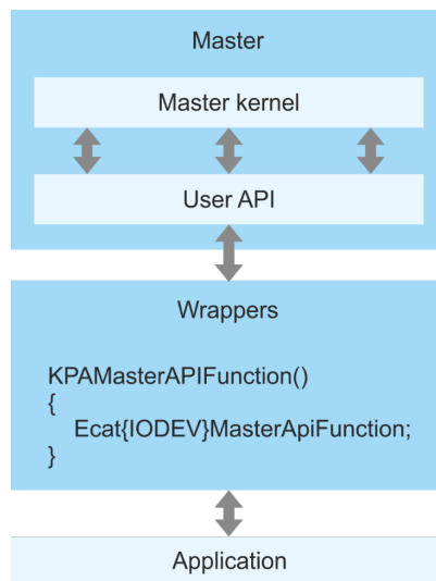
Figure 5. LoadLibrary Function
