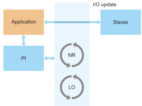
Figure 4. Synchronous 2 mode
