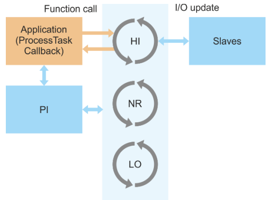
Figure 3. Synchronous 1 mode
